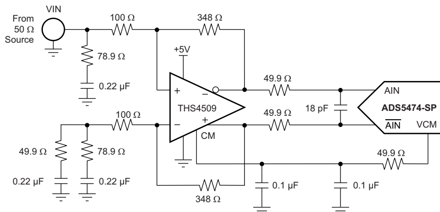
Figure 33. Using the THS4509 or THS4520 With the ADS5474
