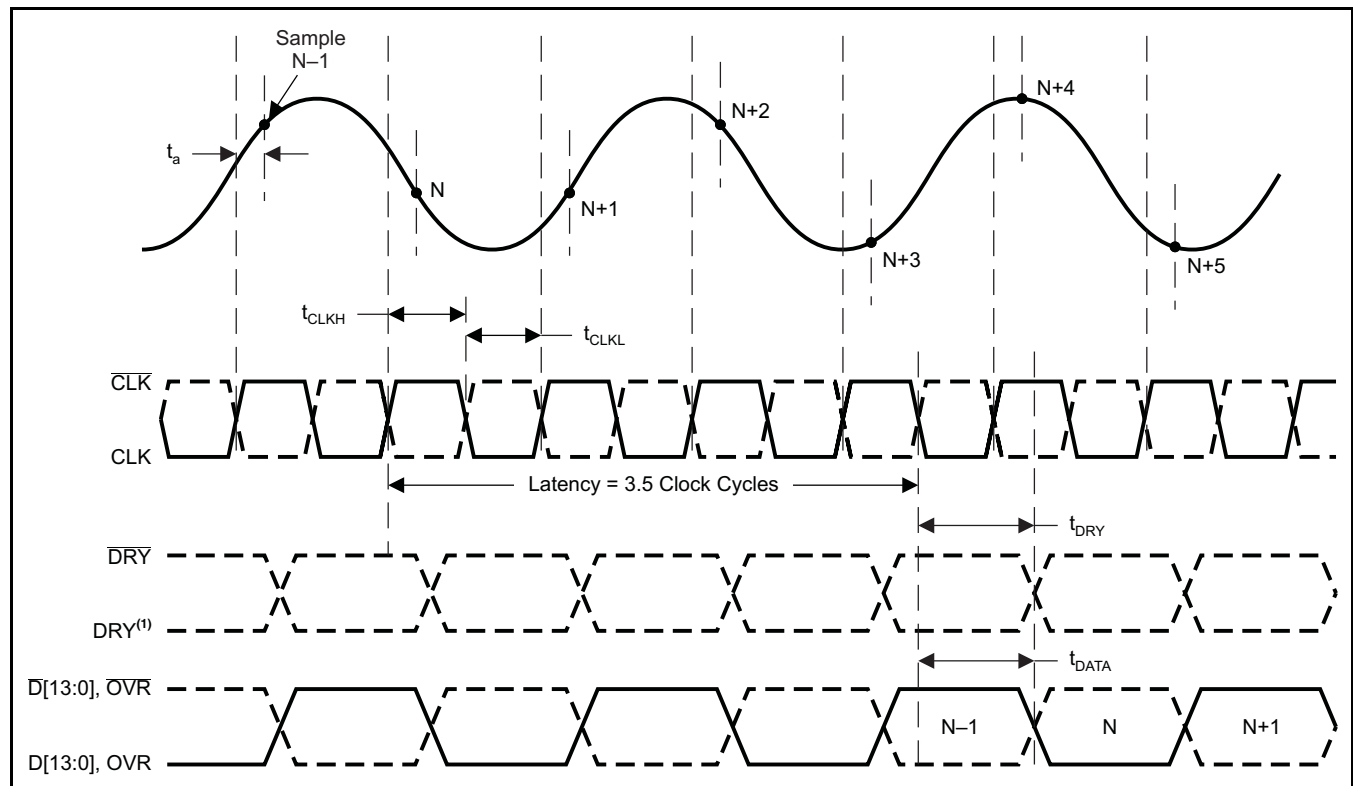
Figure 2. Timing Diagram
